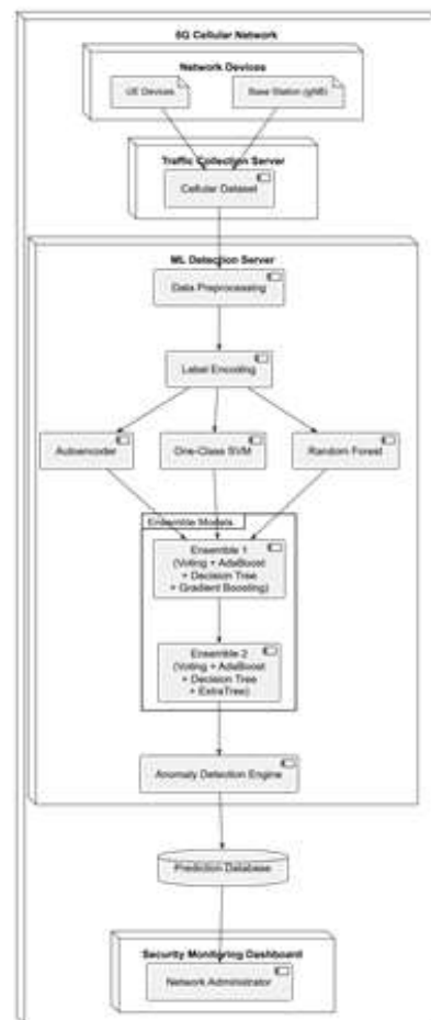
Fig. 2. UML Deployment Diagram for the Machine Learning-Based 5G Network Anomaly Detection Framework
