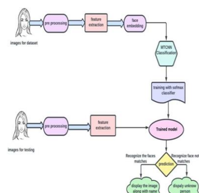
Fig 1. Proposed Method
